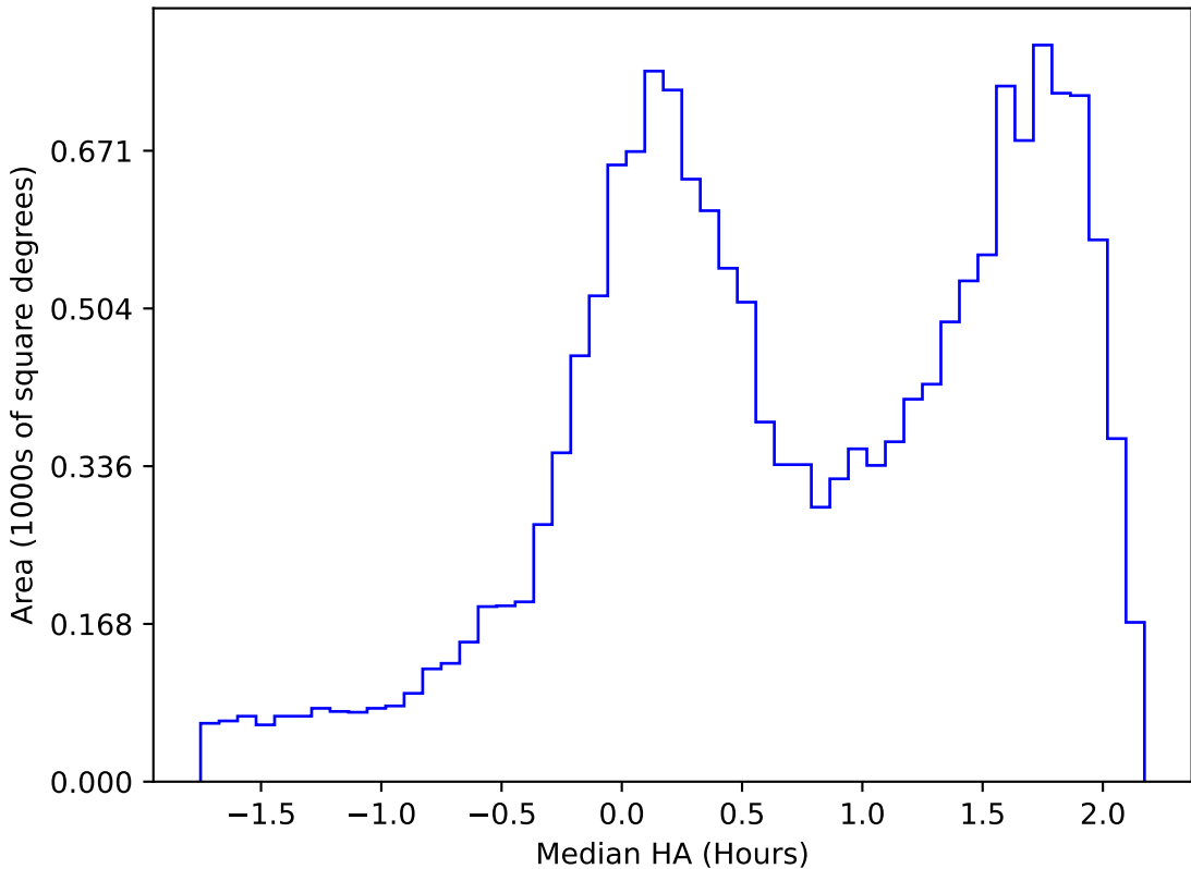
ddf_acor_sf20_lsf40_lsr10_v3.4_10yrs WFD g band: Median HA
