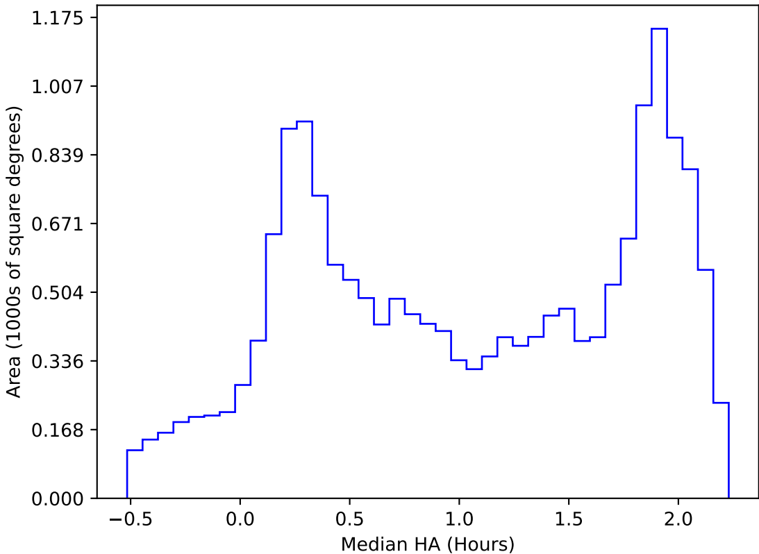
ddf_acor_sf20_lsf40_lsr10_v3.4_10yrs WFD all bands: Median HA
