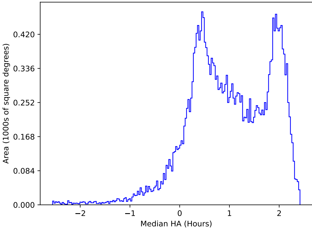
ddf_acor_sf20_lsf40_lsr10_v3.4_10yrs All sky z band: Median HA
