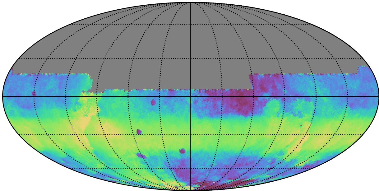
ddf_acor_sf20_lsf40_lsr10_v3.4_10yrs All sky y band: Median HA
