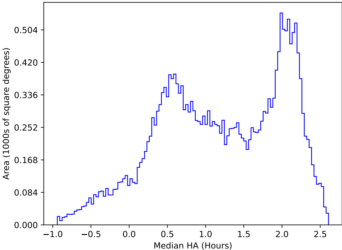
ddf_acor_sf20_lsf40_lsr10_v3.4_10yrs All sky y band: Median HA
