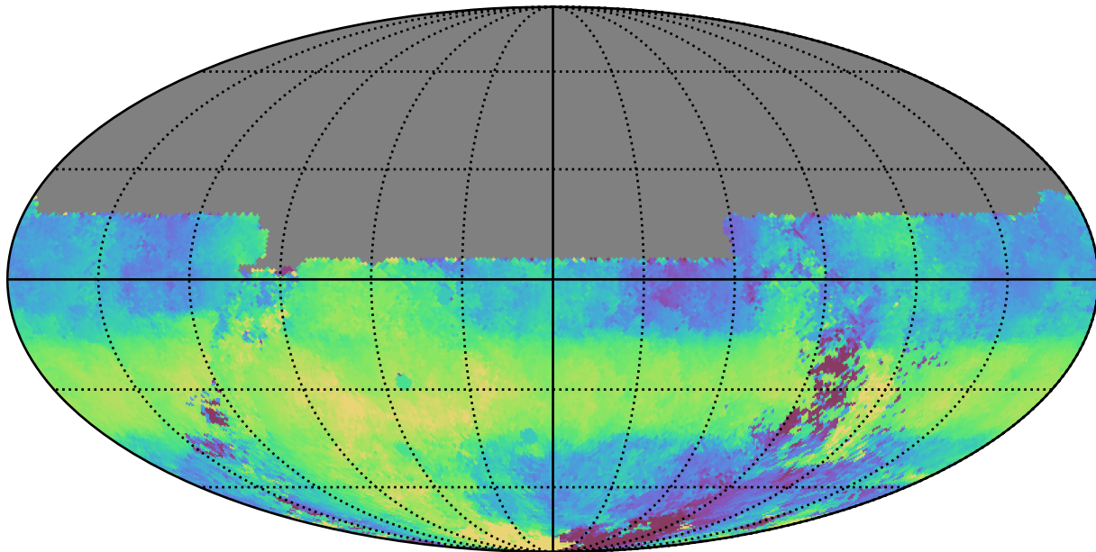
ddf_acor_sf20_lsf40_lsr10_v3.4_10yrs All sky u band: Median HA
