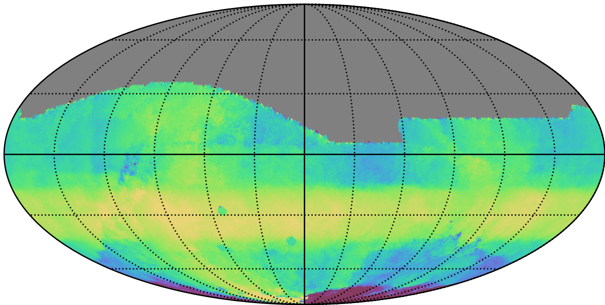
ddf_acor_sf20_lsf40_lsr10_v3.4_10yrs All sky r band: Median HA
