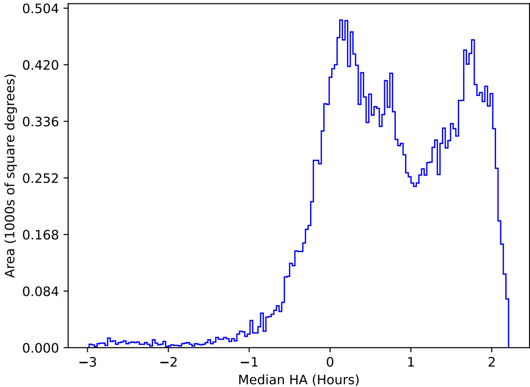
ddf_acor_sf20_lsf40_lsr10_v3.4_10yrs All sky r band: Median HA
