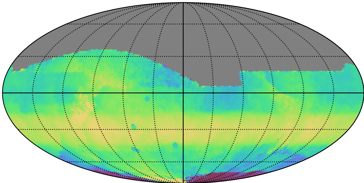
ddf_acor_sf20_lsf40_lsr10_v3.4_10yrs All sky i band: Median HA
