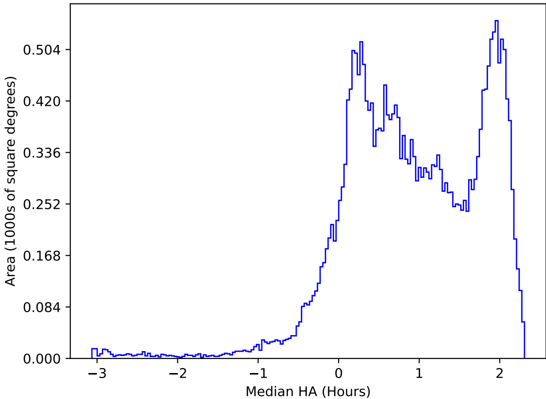
ddf_acor_sf20_lsf40_lsr10_v3.4_10yrs All sky i band: Median HA
