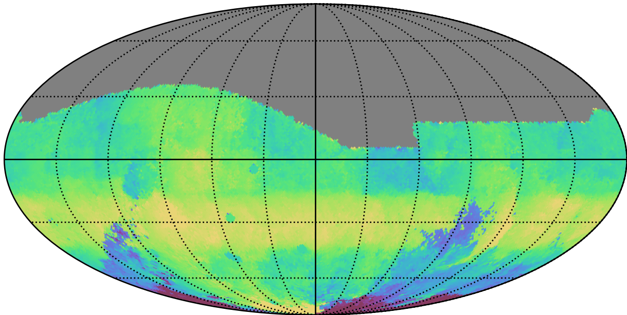
ddf_acor_sf20_lsf40_lsr10_v3.4_10yrs All sky g band: Median HA
