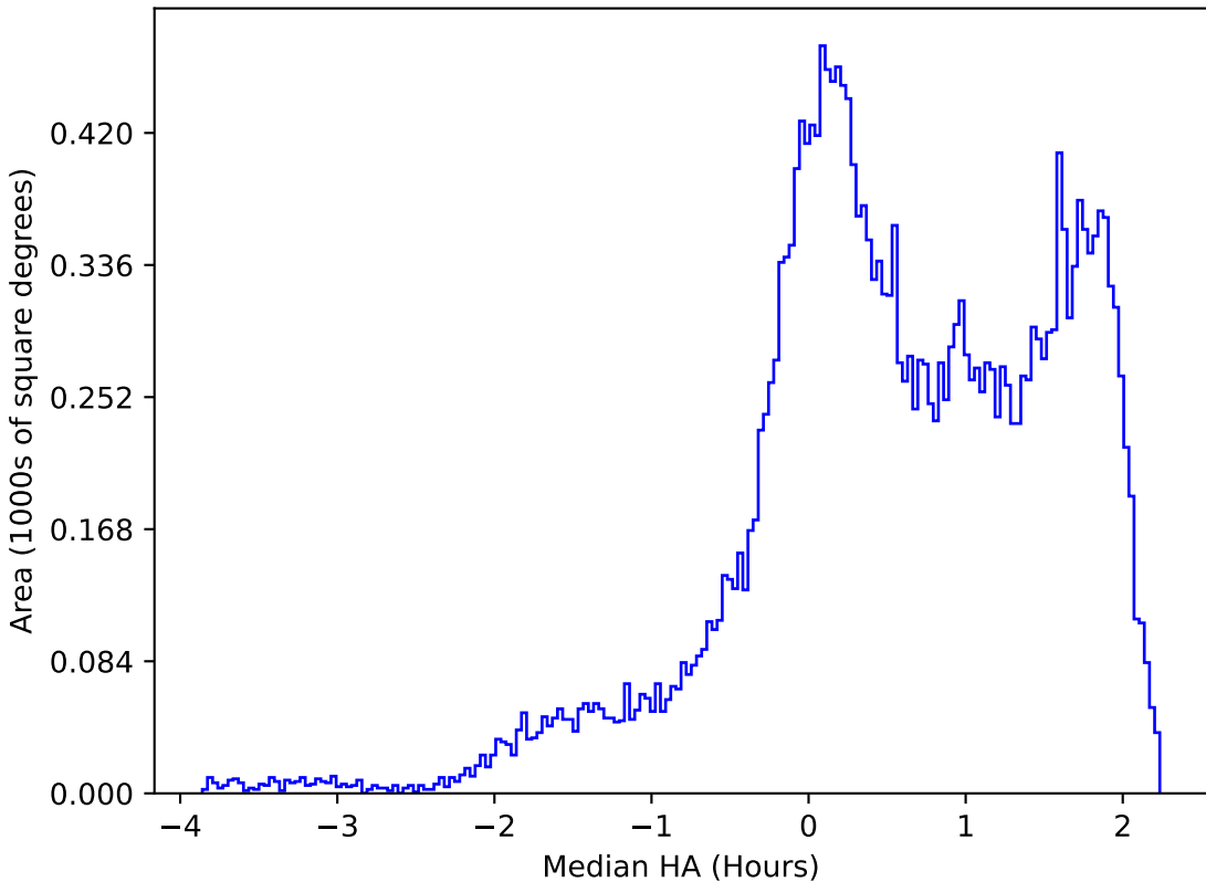
ddf_acor_sf20_lsf40_lsr10_v3.4_10yrs All sky g band: Median HA
