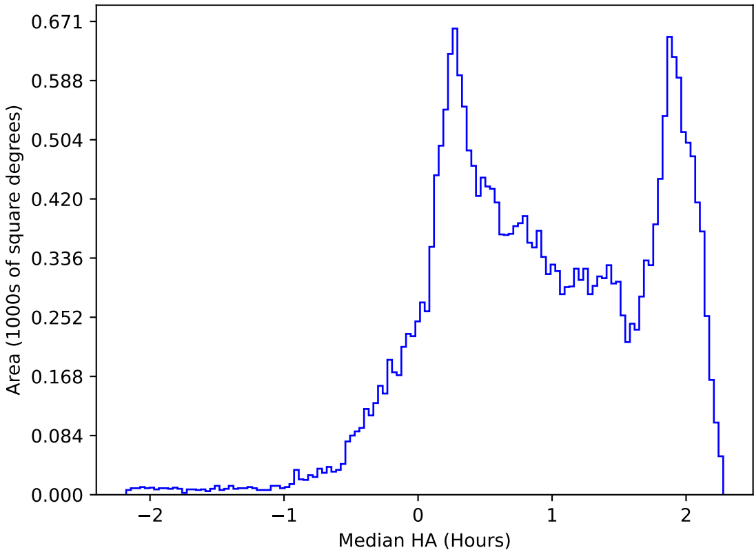
ddf_acor_sf20_lsf40_lsr10_v3.4_10yrs All sky all bands: Median HA
