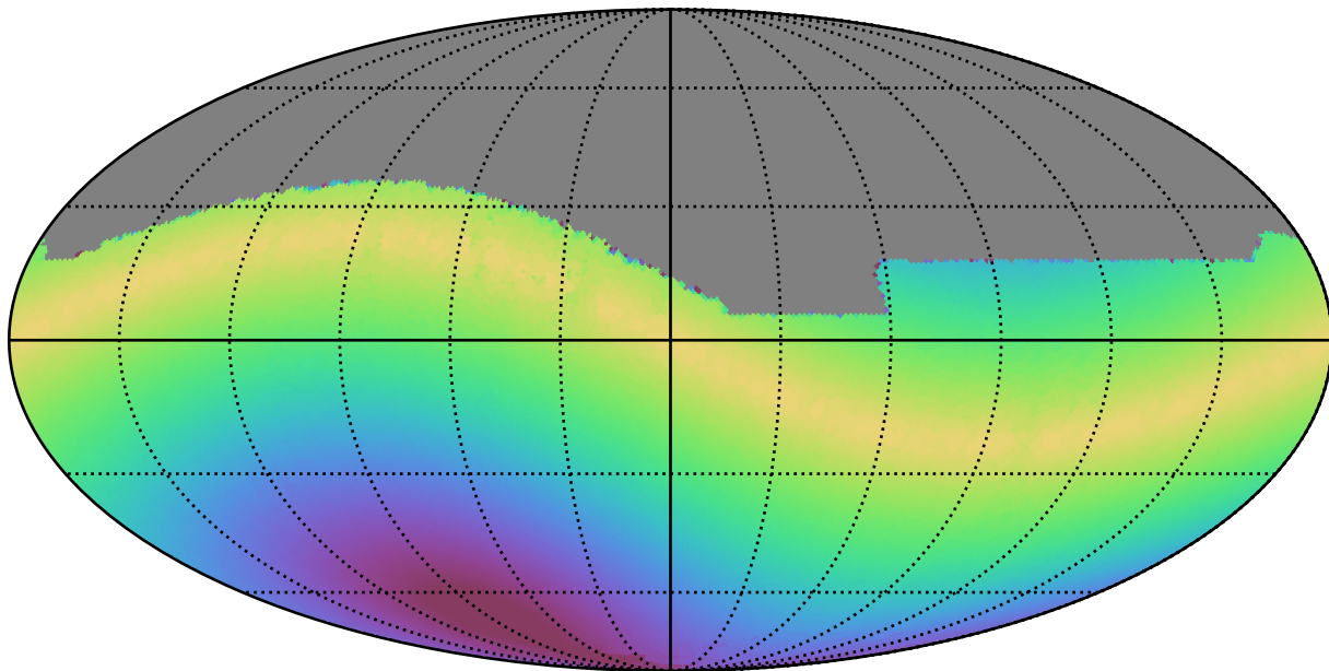
ddf_acor_sf20_lsf40_lsr10_v3.4_10yrs All sky i band: Max solarElong
