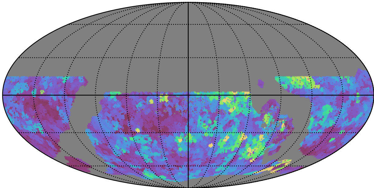
ddf_acor_sf20_lsf40_lsr10_v3.4_10yrs WFD u band: Max seeingEff
