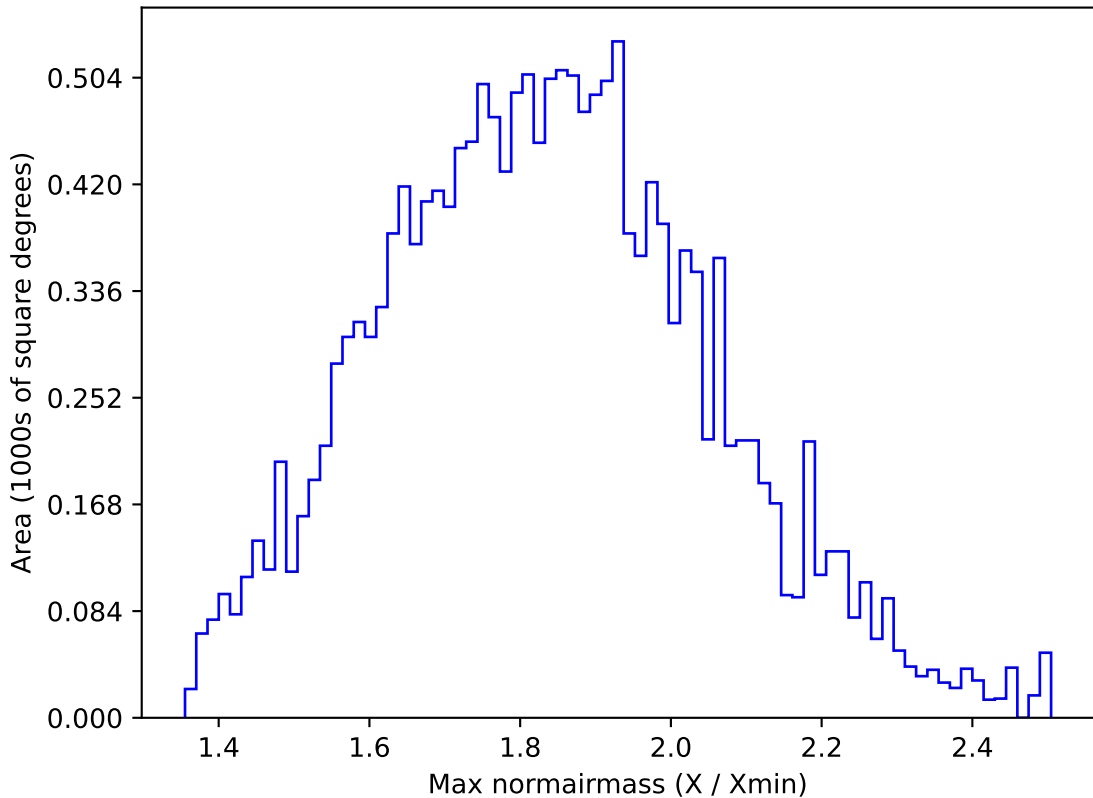
ddf_acor_sf20_lsf40_lsr10_v3.4_10yrs WFD g band: Max normairmass
