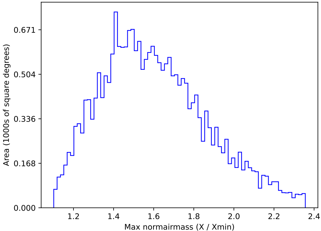
ddf_acor_sf20_lsf40_lsr10_v3.4_10yrs All sky u band: Max normairmass
