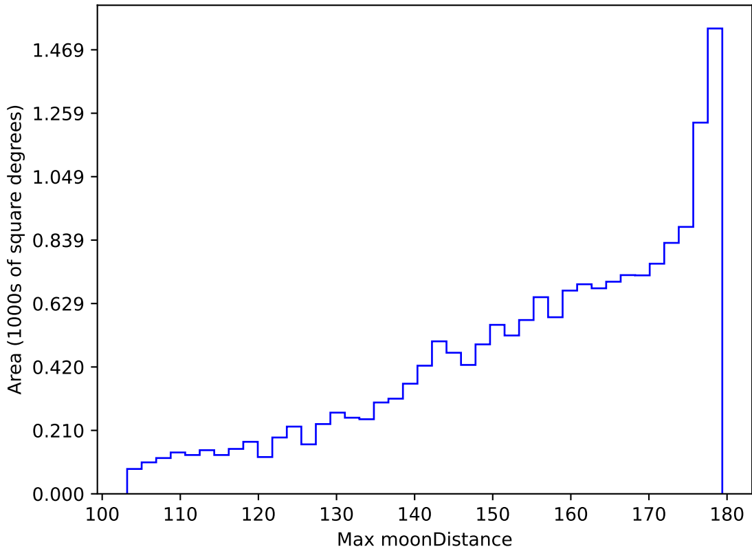
ddf_acor_sf20_lsf40_lsr10_v3.4_10yrs WFD r band: Max moonDistance
