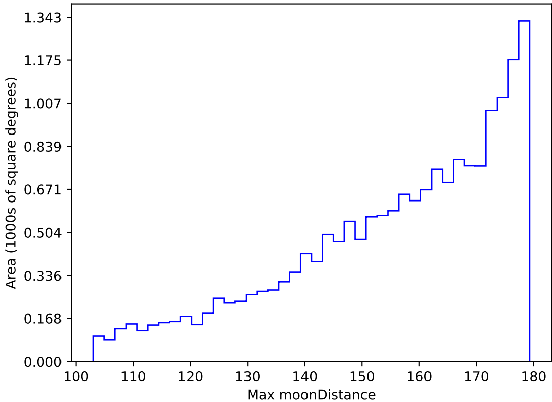
ddf_acor_sf20_lsf40_lsr10_v3.4_10yrs WFD i band: Max moonDistance
