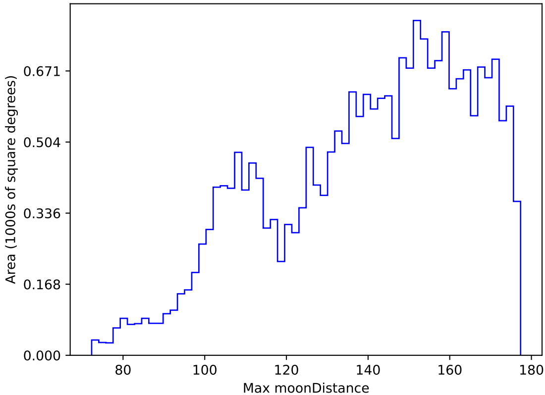
ddf_acor_sf20_lsf40_lsr10_v3.4_10yrs All sky y band: Max moonDistance
