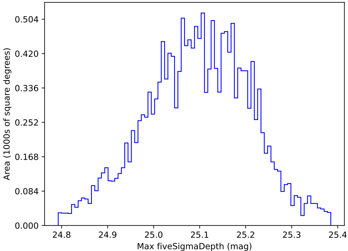
ddf_acor_sf20_lsf40_lsr10_v3.4_10yrs WFD all bands: Max fiveSigmaDepth
