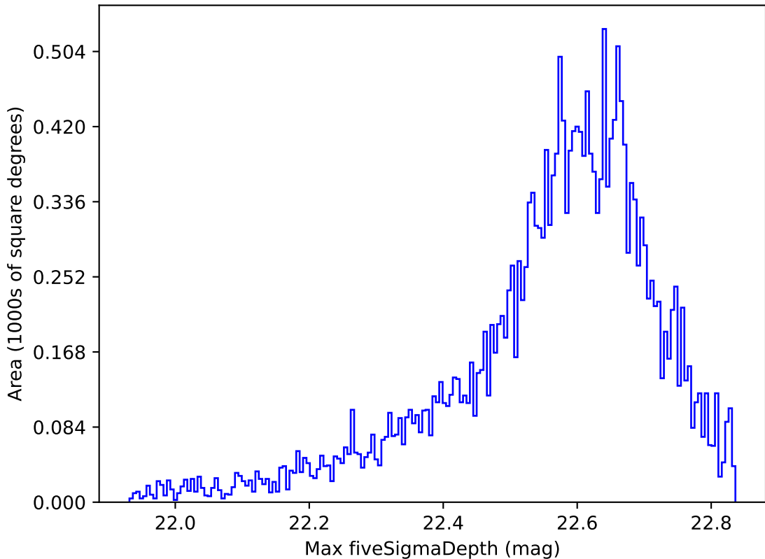
ddf_acor_sf20_lsf40_lsr10_v3.4_10yrs All sky y band: Max fiveSigmaDepth
