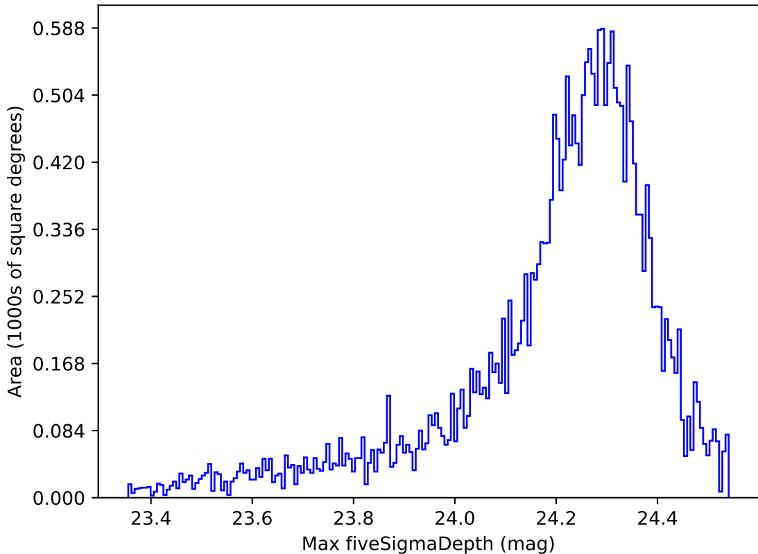
ddf_acor_sf20_lsf40_lsr10_v3.4_10yrs All sky i band: Max fiveSigmaDepth
