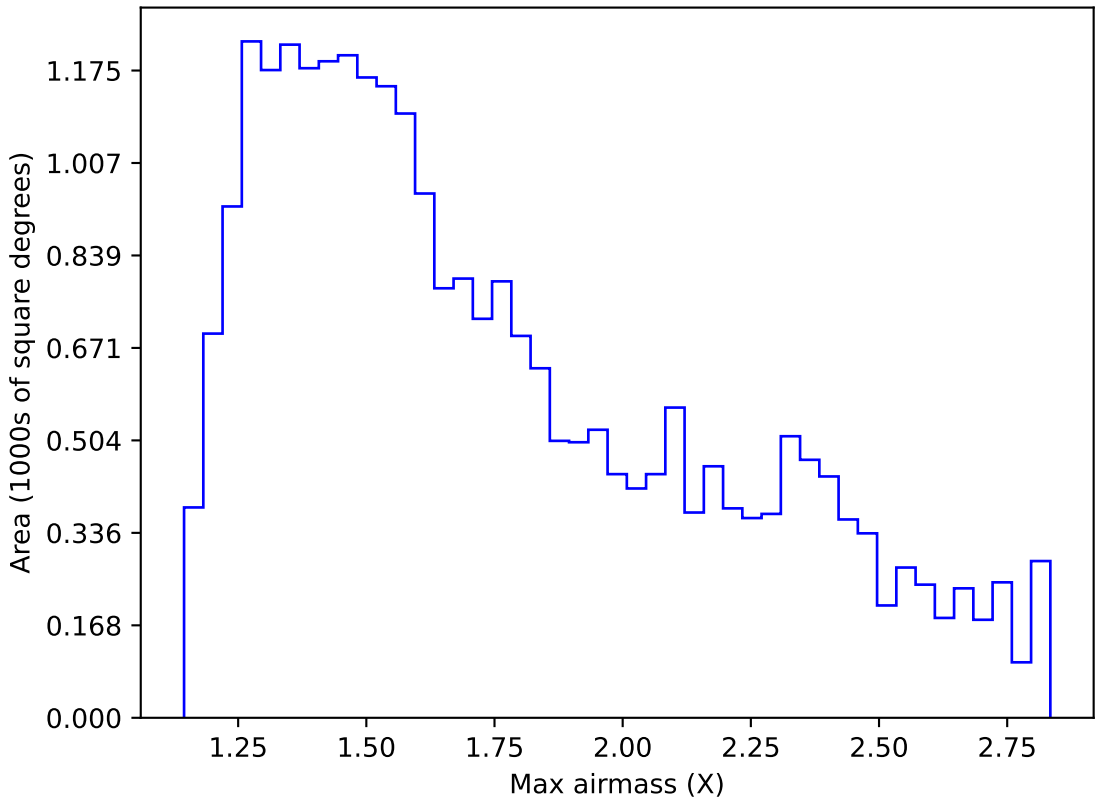
ddf_acor_sf20_lsf40_lsr10_v3.4_10yrs Yr 1 z band: Max airmass
