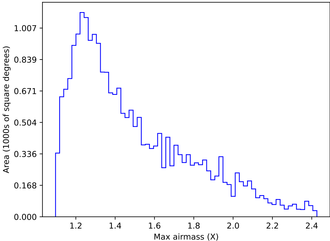
ddf_acor_sf20_lsf40_lsr10_v3.4_10yrs Yr 1 u band: Max airmass
