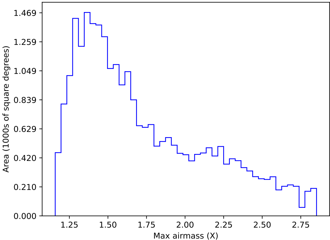
ddf_acor_sf20_lsf40_lsr10_v3.4_10yrs Yr 1 i band: Max airmass
