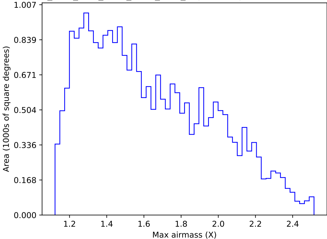
ddf_acor_sf20_lsf40_lsr10_v3.4_10yrs Yr 1 g band: Max airmass
