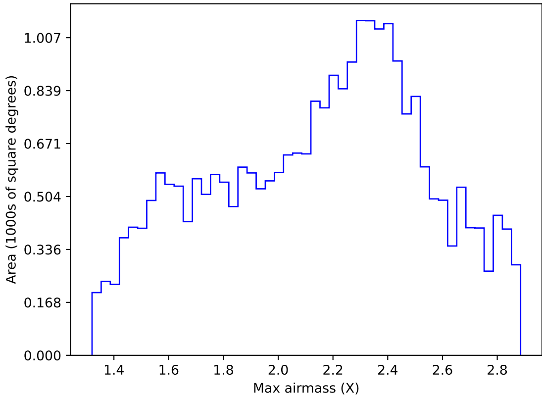
ddf_acor_sf20_lsf40_lsr10_v3.4_10yrs Yr 1 all bands: Max airmass
