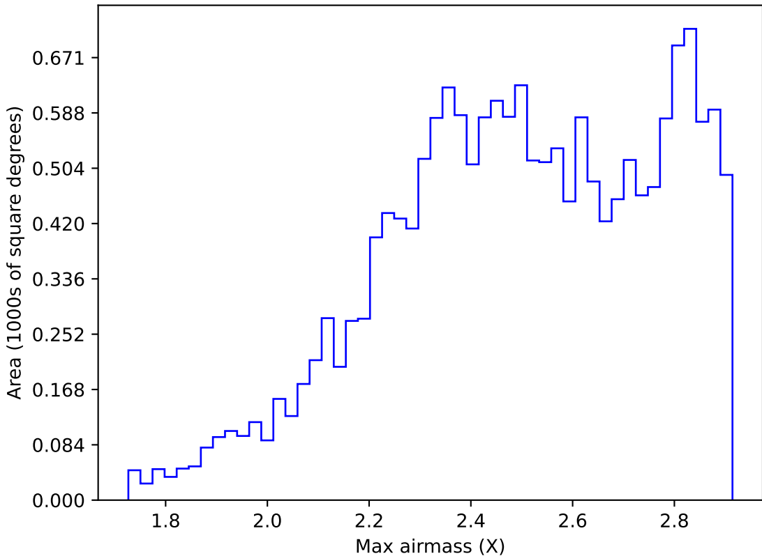
ddf_acor_sf20_lsf40_lsr10_v3.4_10yrs WFD z band: Max airmass
