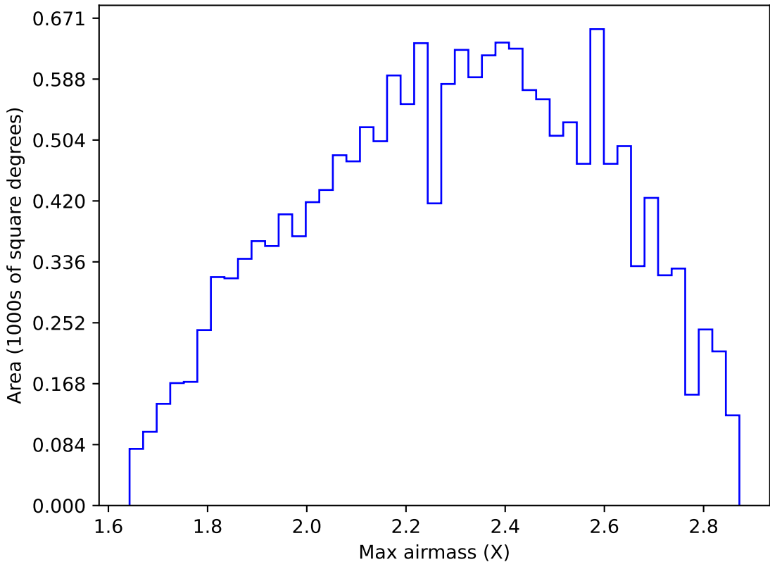
ddf_acor_sf20_lsf40_lsr10_v3.4_10yrs WFD y band: Max airmass
