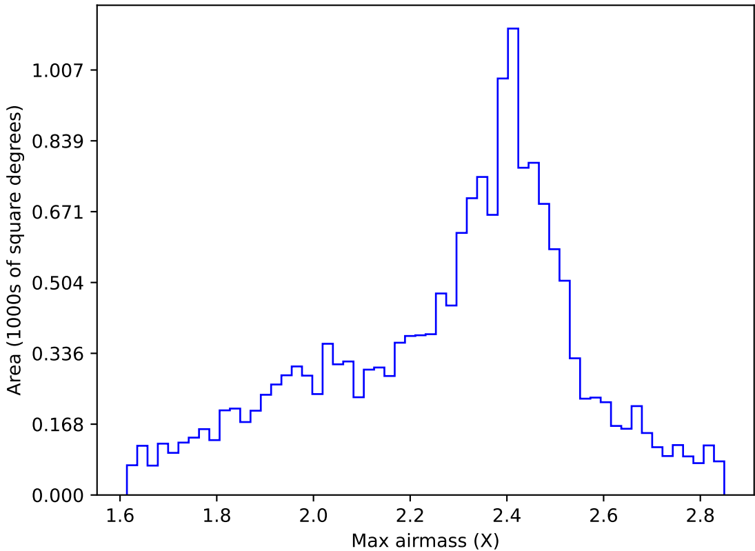
ddf_acor_sf20_lsf40_lsr10_v3.4_10yrs WFD r band: Max airmass
