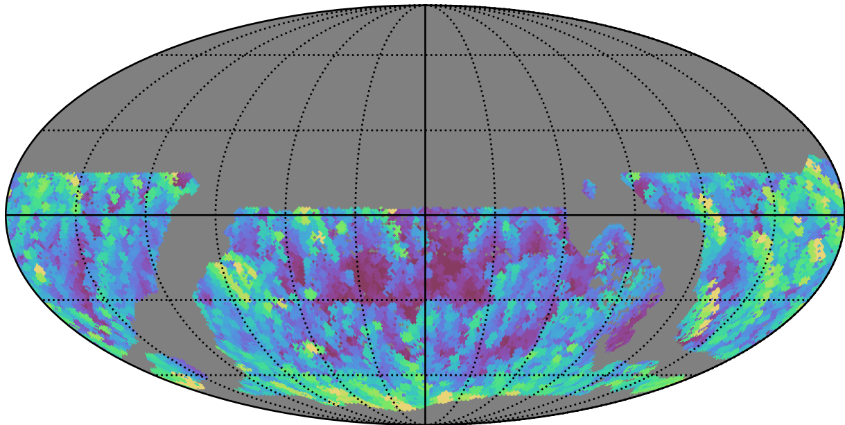
ddf_acor_sf20_lsf40_lsr10_v3.4_10yrs WFD g band: Max airmass
