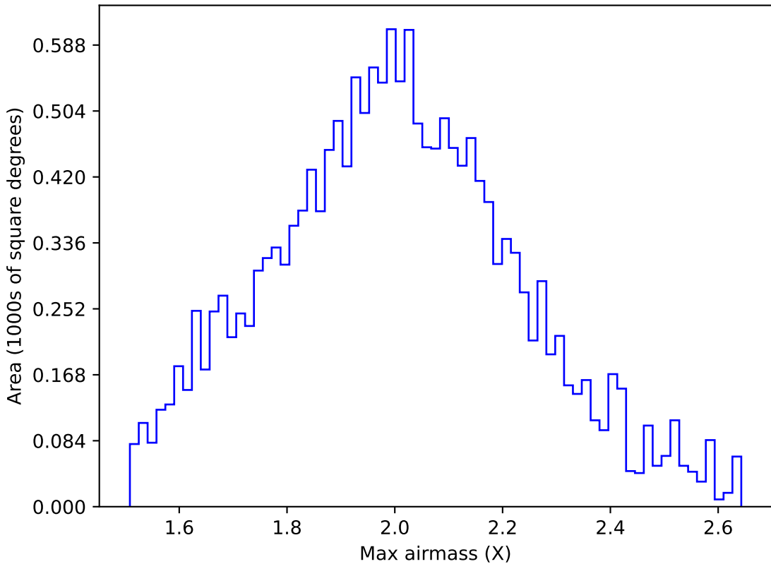
ddf_acor_sf20_lsf40_lsr10_v3.4_10yrs WFD g band: Max airmass
