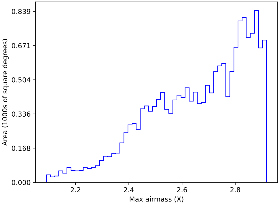
ddf_acor_sf20_lsf40_lsr10_v3.4_10yrs WFD all bands: Max airmass
