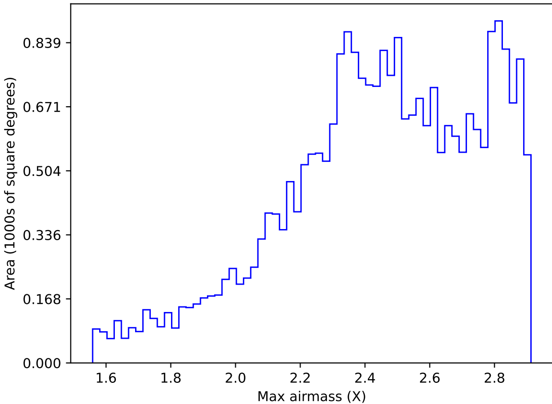
ddf_acor_sf20_lsf40_lsr10_v3.4_10yrs All sky z band: Max airmass
