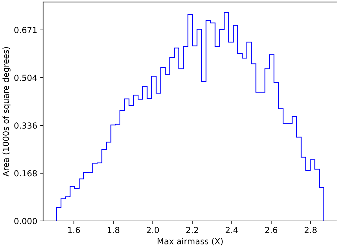
ddf_acor_sf20_lsf40_lsr10_v3.4_10yrs All sky y band: Max airmass
