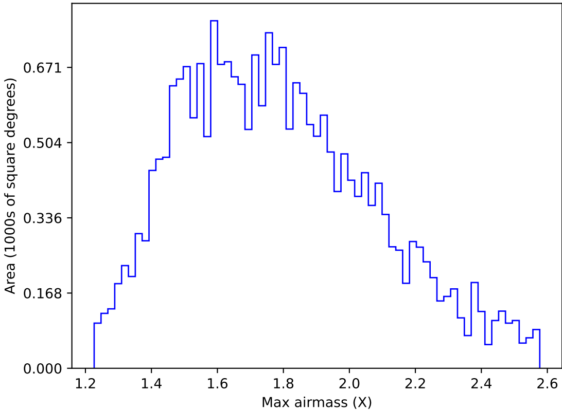
ddf_acor_sf20_lsf40_lsr10_v3.4_10yrs All sky u band: Max airmass
