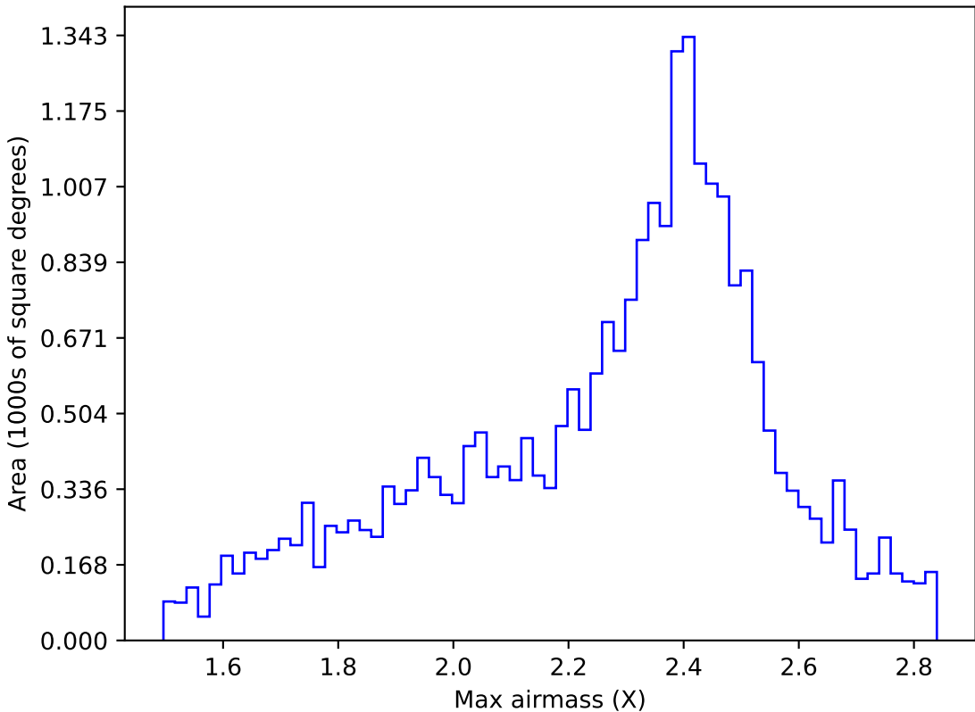
ddf_acor_sf20_lsf40_lsr10_v3.4_10yrs All sky r band: Max airmass
