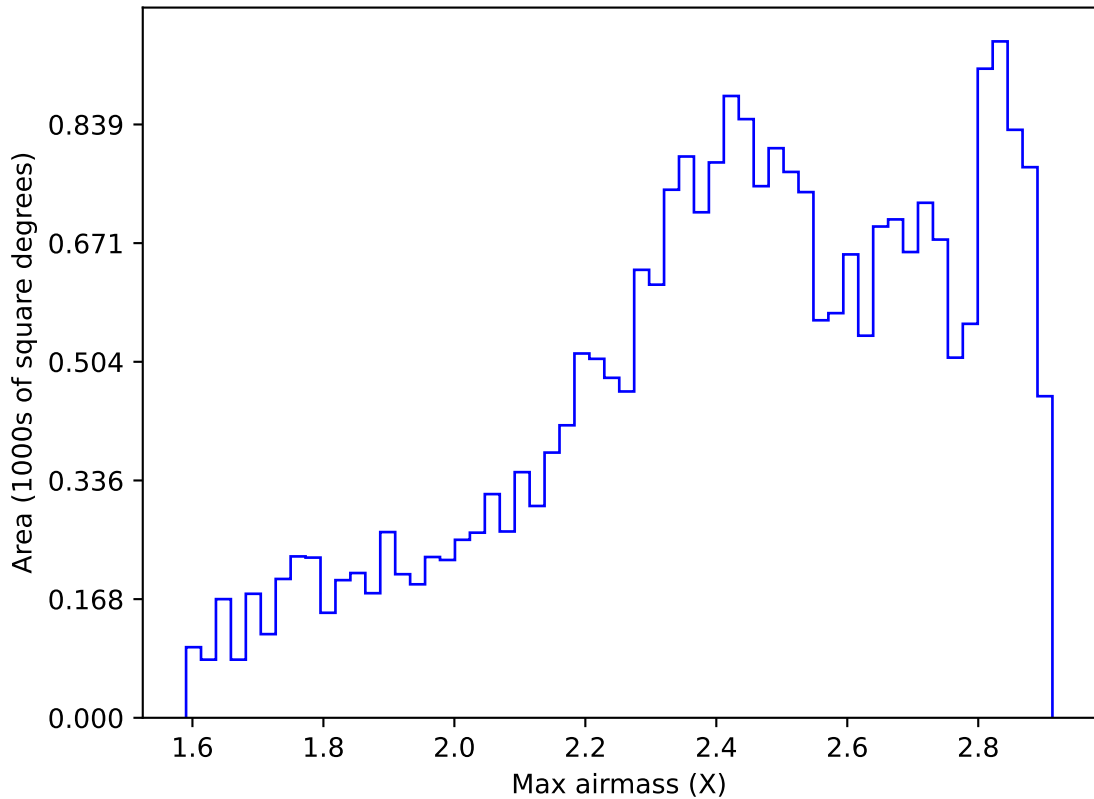
ddf_acor_sf20_lsf40_lsr10_v3.4_10yrs All sky i band: Max airmass
