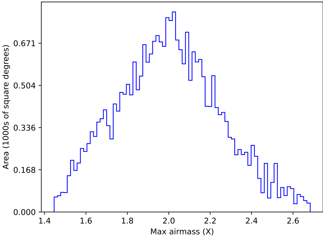
ddf_acor_sf20_lsf40_lsr10_v3.4_10yrs All sky g band: Max airmass
