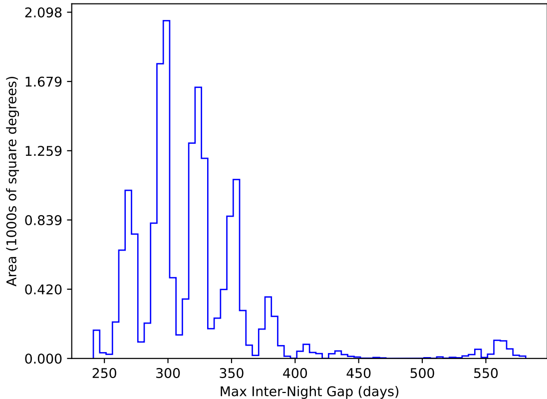
ddf_acor_sf20_lsf40_lsr10_v3.4_10yrs WFD y band: Max Inter-Night Gap
