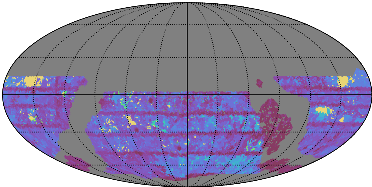
ddf_acor_sf20_lsf40_lsr10_v3.4_10yrs WFD r band: Max Inter-Night Gap
