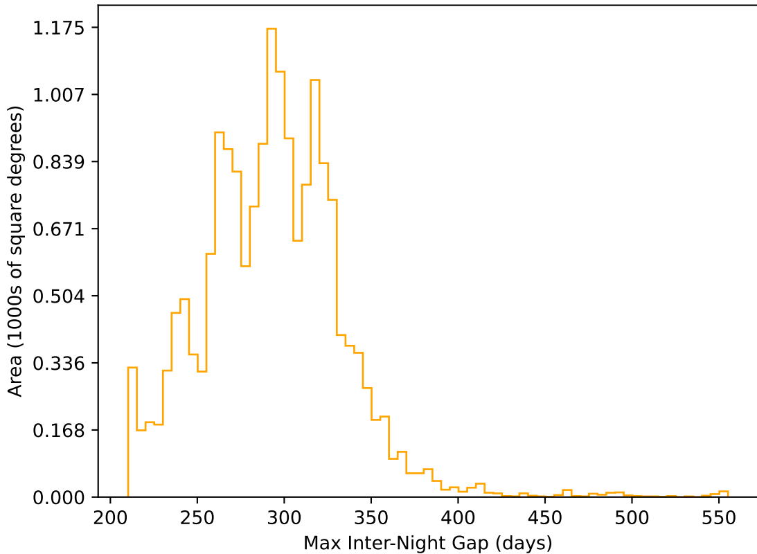
ddf_acor_sf20_lsf40_lsr10_v3.4_10yrs WFD r band: Max Inter-Night Gap
