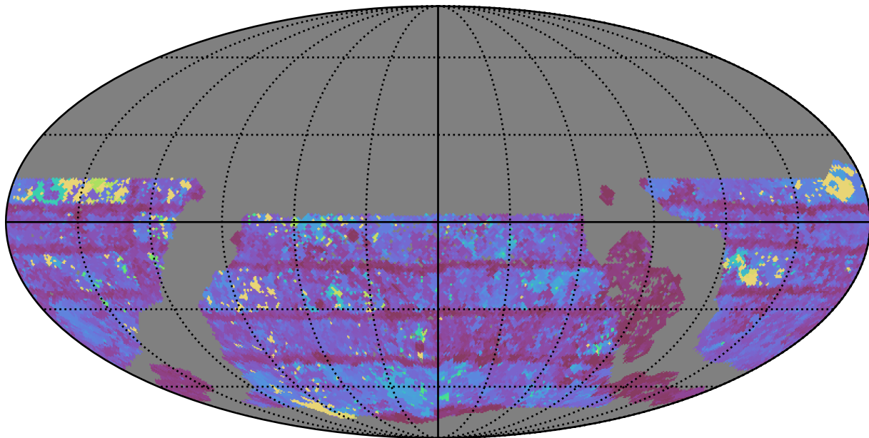
ddf_acor_sf20_lsf40_lsr10_v3.4_10yrs WFD i band: Max Inter-Night Gap
