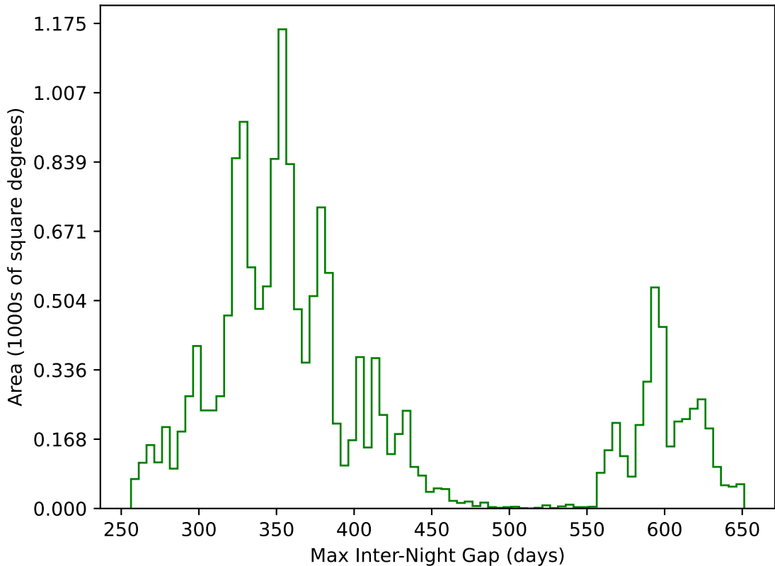
ddf_acor_sf20_lsf40_lsr10_v3.4_10yrs WFD g band: Max Inter-Night Gap
