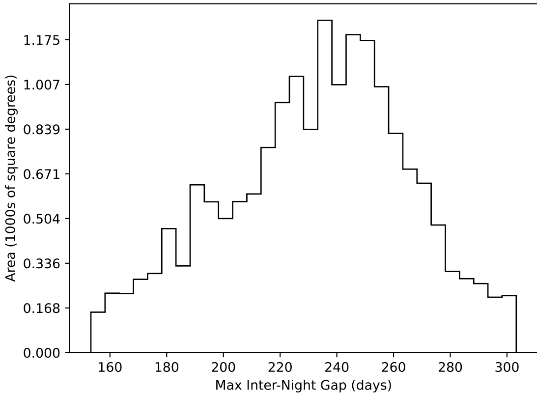
ddf_acor_sf20_lsf40_lsr10_v3.4_10yrs WFD all bands: Max Inter-Night Gap
