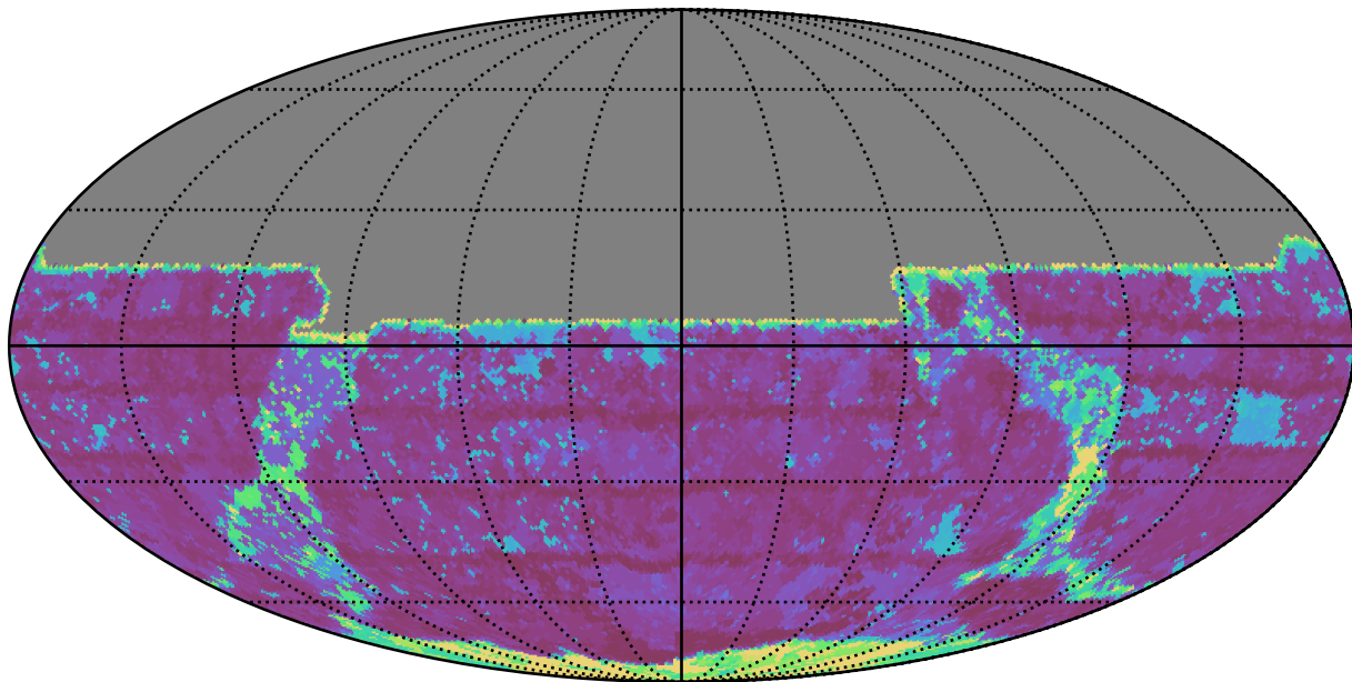
ddf_acor_sf20_lsf40_lsr10_v3.4_10yrs All sky y band: Max Inter-Night Gap
