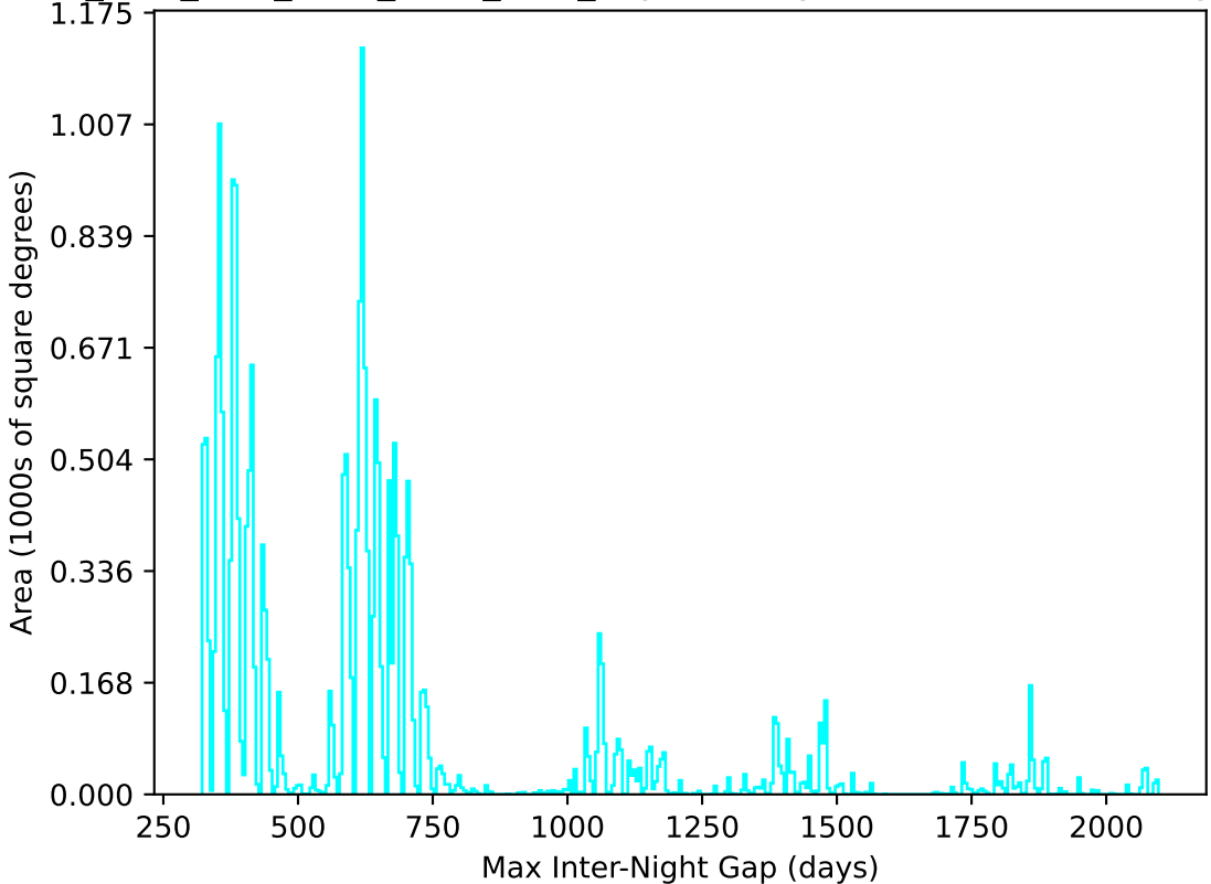
ddf_acor_sf20_lsf40_lsr10_v3.4_10yrs All sky u band: Max Inter-Night Gap
