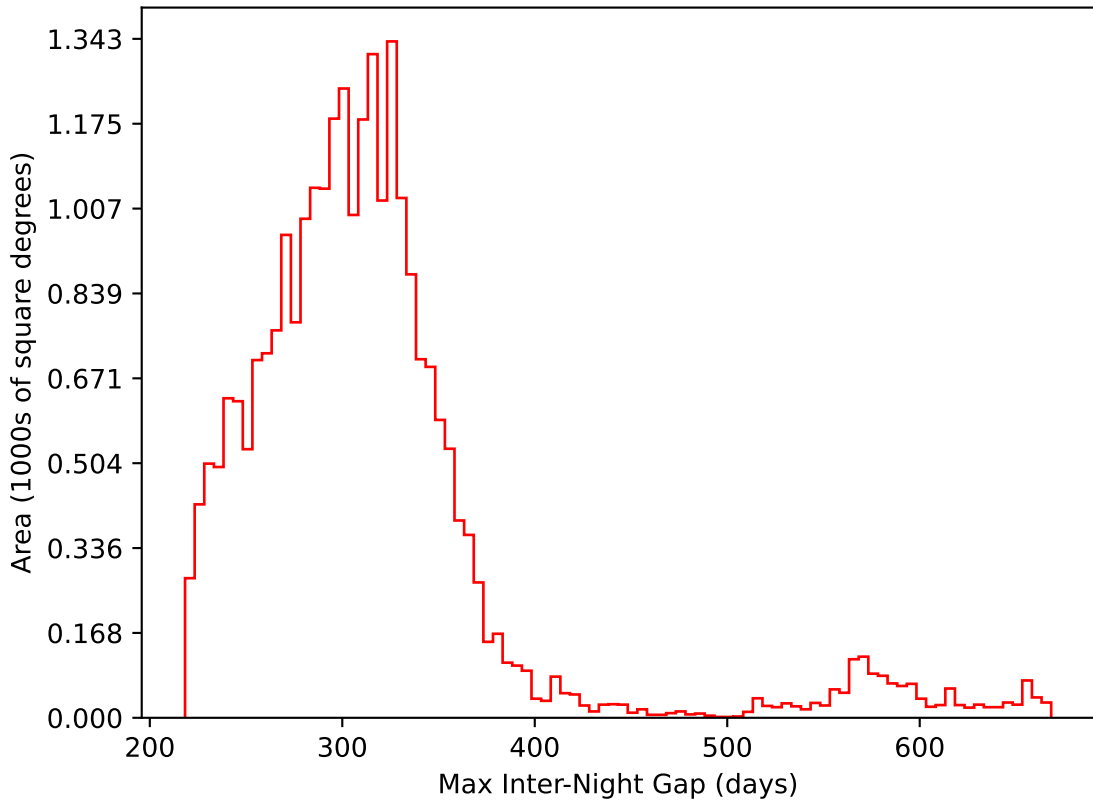
ddf_acor_sf20_lsf40_lsr10_v3.4_10yrs All sky i band: Max Inter-Night Gap
