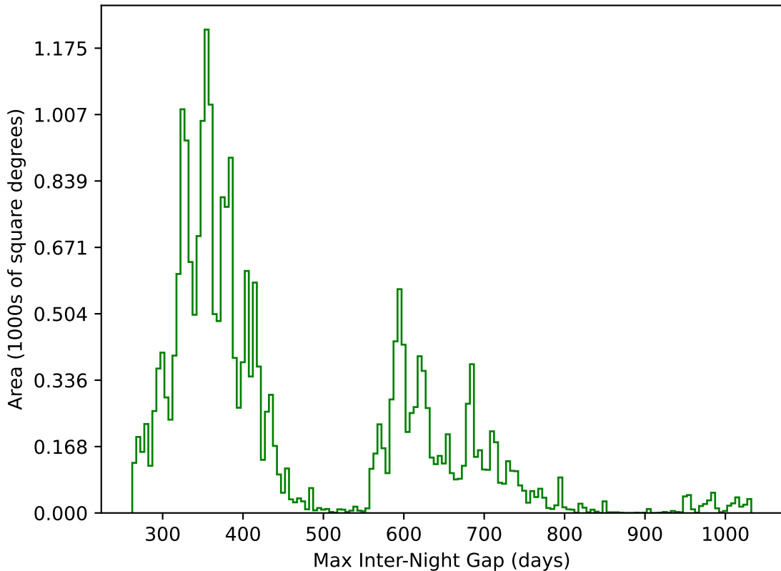
ddf_acor_sf20_ls40_lsr10_v3.4_10yrs All sky g band: Max Inter-Night Gap
